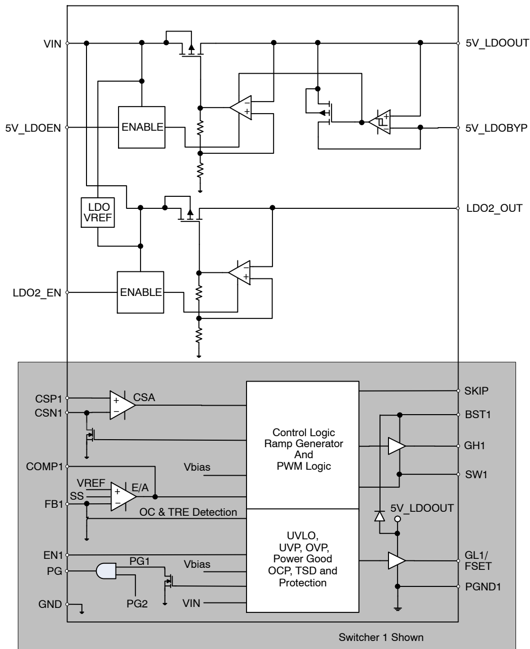
Figure 1. Block Diagram
