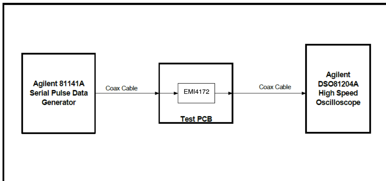
Figure 6. EMI4172 Eye Diagram Test Setup
