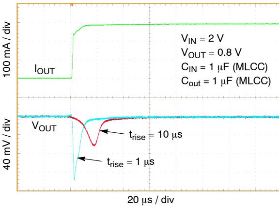
Figure 43. Load Transient Response – Rising Edge, V_{OUT} = 0.8 \text{ V} , I_{OUT} = 1 \text{ mA} to 300 mA, t_{RISE} = 1 \mu\text{s} , 10 \mu\text{s}
