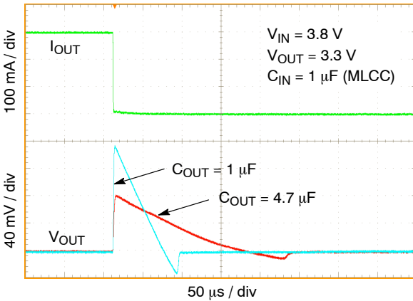
Figure 45. Load Transient Response – Falling Edge, V_{OUT} = 3.3 \text{ V} , I_{OUT} = 1 \text{ mA} to 300 mA, C_{OUT} = 1 \mu\text{F} , 4.7 \mu\text{F}
