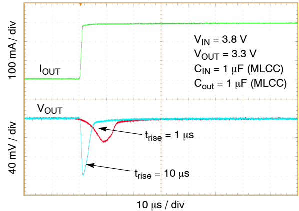
Figure 46. Load Transient Response – Rising Edge, V_{OUT} = 3.3 \text{ V} , I_{OUT} = 1 \text{ mA} to 300 mA, t_{RISE} = 1 \mu\text{s} , 10 \mu\text{s}
