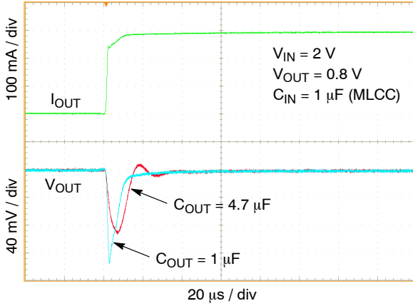
Figure 41. Load Transient Response – Rising Edge, V_{OUT} = 0.8 \text{ V} , I_{OUT} = 1 \text{ mA} to 300 mA, C_{OUT} = 1 \mu\text{F} , 4.7 \mu\text{F}
