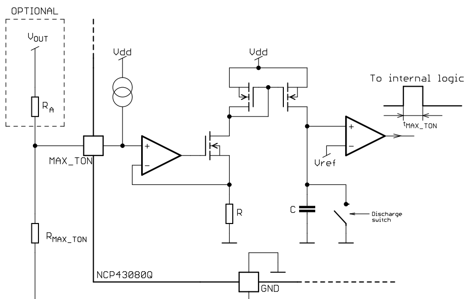
Figure 50. Internal Connection of the MAX TON Generator, NCP43080Q
