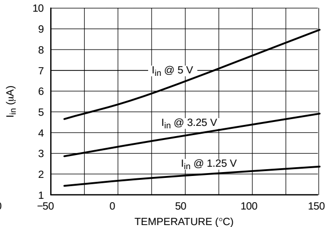
Figure 12. Input Current vs. Temperature
