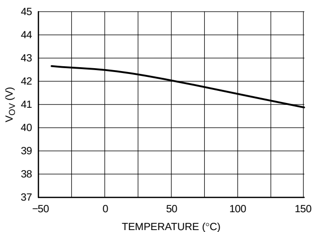
Figure 6. Overvoltage Shutdown vs. Temperature
