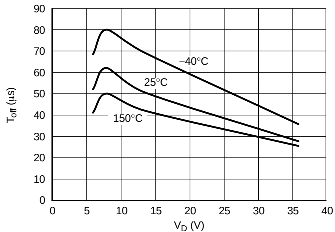
Figure 16. Turn Off Time vs. V D
