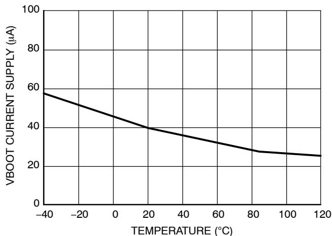
Figure 41. V_{BOOT} Supply Current vs. Temperature
