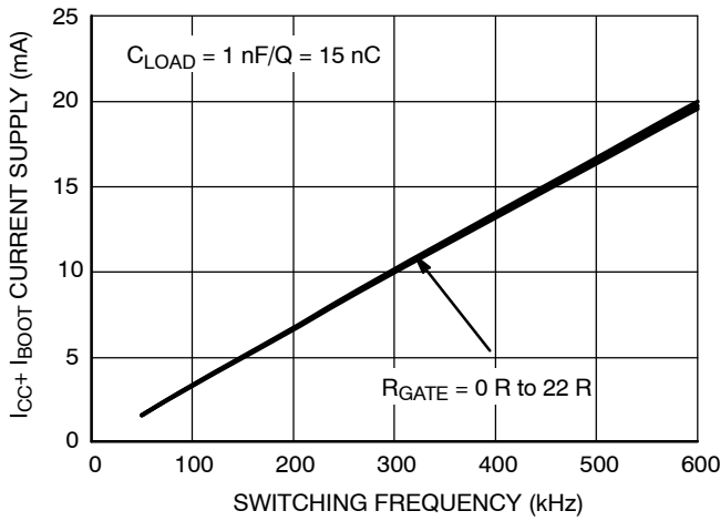
Figure 46. I_{CC1} Consumption vs. Switching Frequency with 15 nC Load on Each Driver @ V_{CC} = 15\text{ V}
