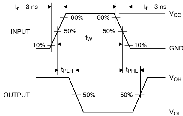
Figure 7. AC Waveforms
