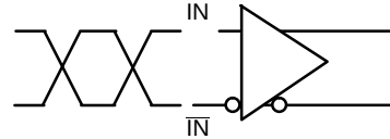
Figure 23. Differential Inputs Driven Differentially
