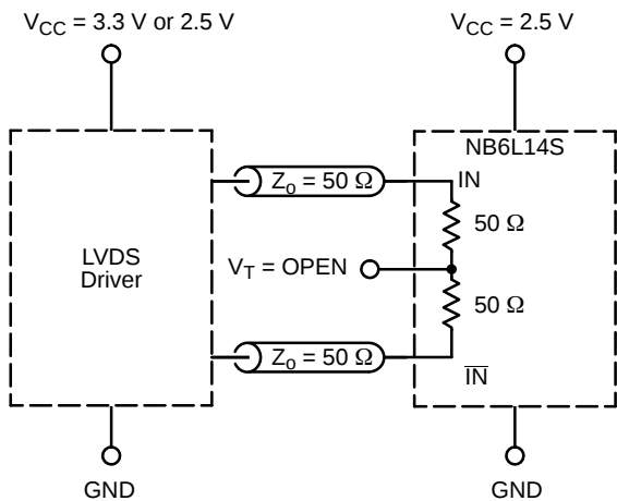
Figure 12. LVDS Interface
