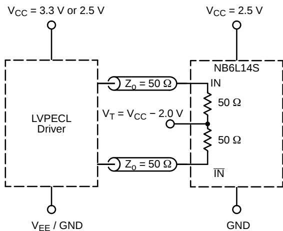
Figure 10. LVPECL Interface
