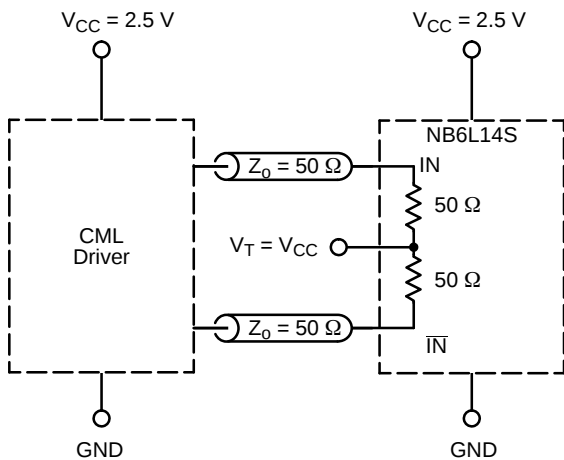
Figure 13. CML Interface
