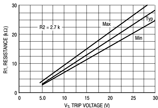
Figure 9. R1 versus Trip Voltage
