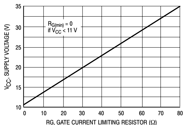
Figure 10. Minimum R_G versus Supply Voltage
