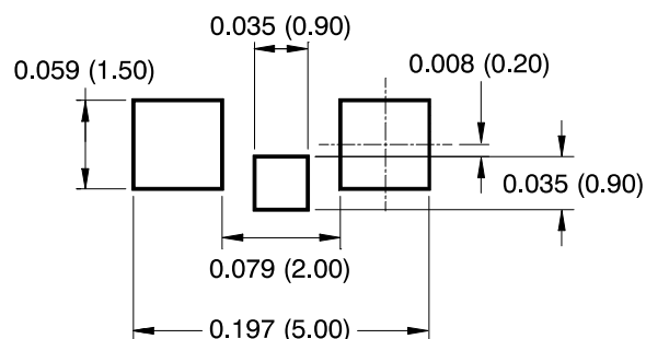
FOOTPRINT
