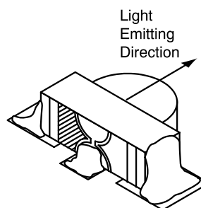
MOUNTING EXAMPLE
