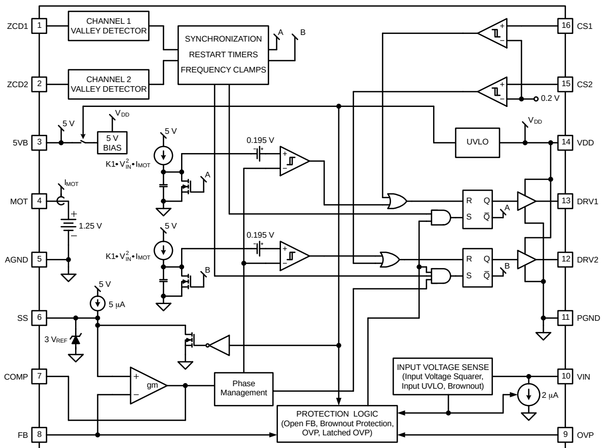
Figure 4. Block Diagram
