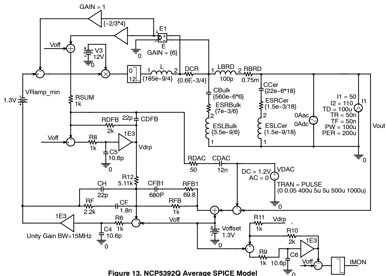
Figure 13. NCP5392Q Average SPICE Model
