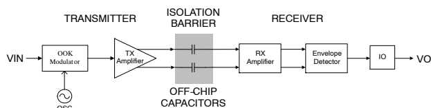
Figure 11. Operational Block Diagram of Single Channel
