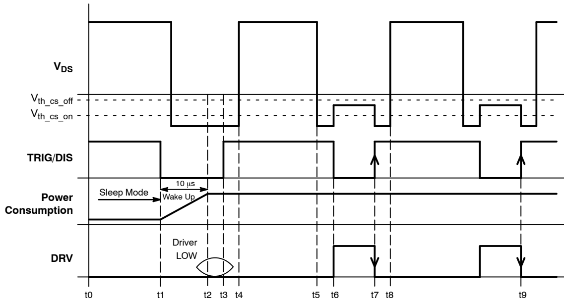
Figure 57. Waking-up Sequence
