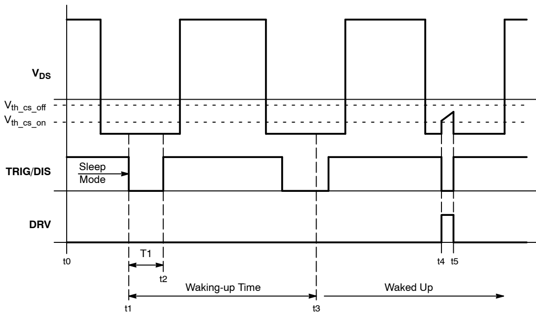
Figure 58. Wake-up Time Sequence
