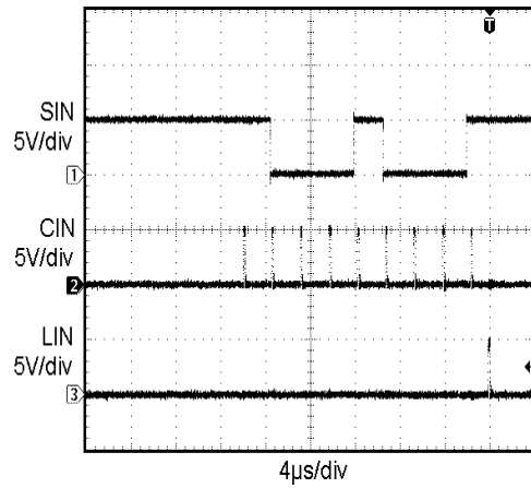
Figure 15. Programming Example
