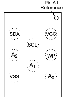
WLCSP (C8A) (Top View)
