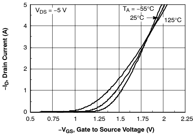
Figure 5. Transfer Characteristics
