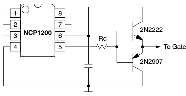
Figure 26. Improving Both Turn-On and Turn-Off Times
