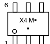
SC-88 W1 SUFFIX CASE 419B
