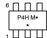
TSOP-6 CASE 318G STYLE 12
