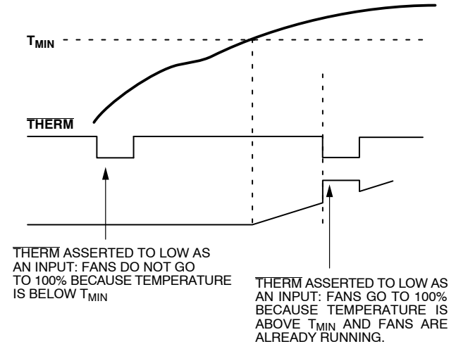
Figure 32. Asserting THERM Low as an Input in Automatic Fan Speed Control Mode
