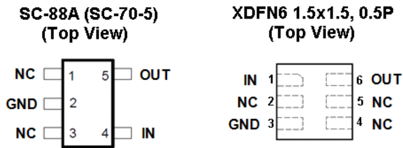
Figure 3. Pin Description
