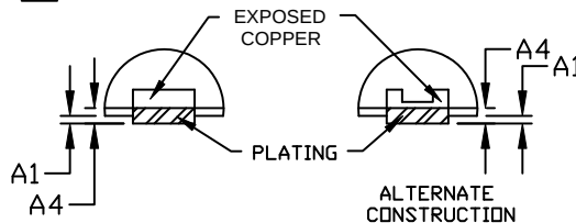
DETAIL B
