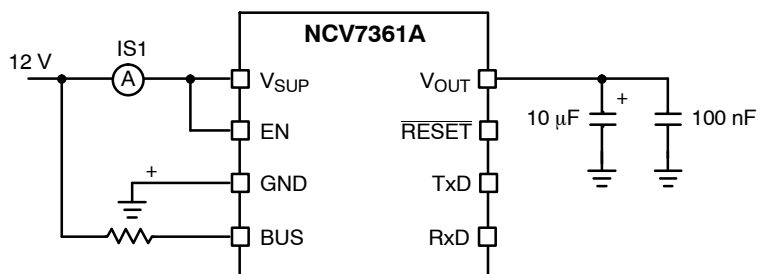
Figure 6. Test Circuit for Supply Current I_{SNL}
