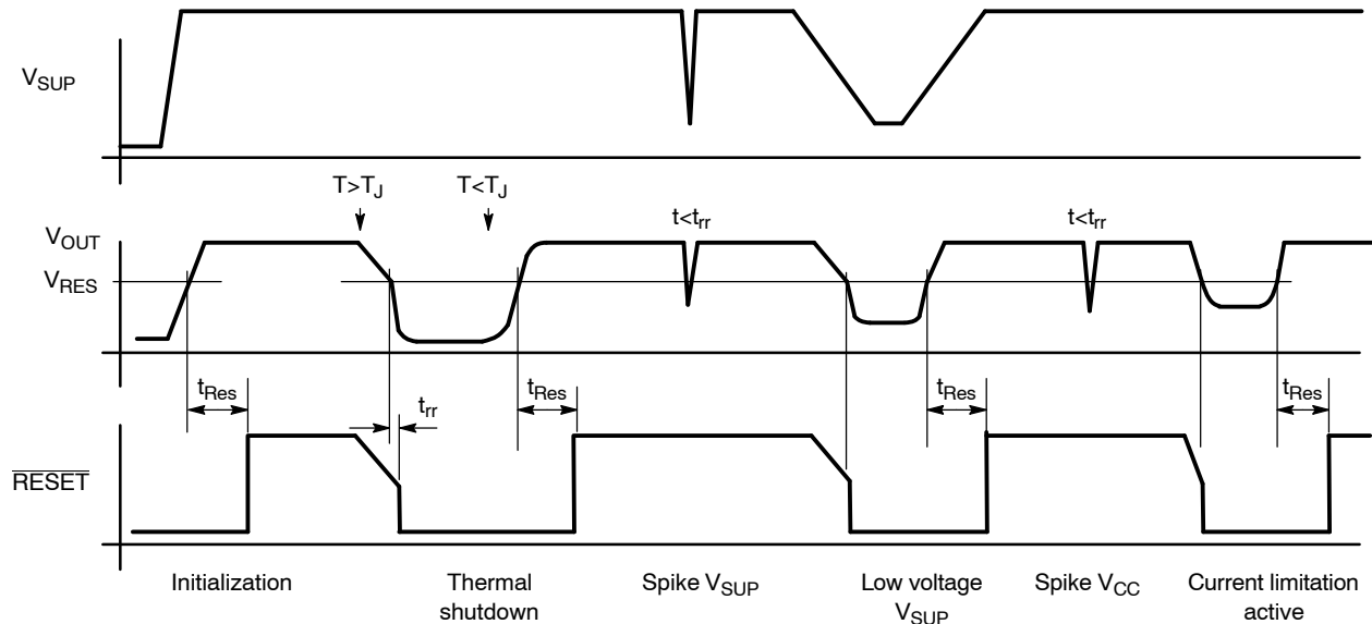
Figure 17. RESET Behavior
