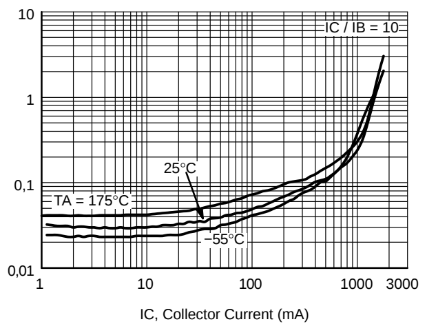
Figure 7. V_{CE(sat)} - I_C
