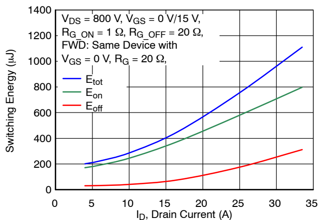
Figure 20. Clamped Inductive Switching Energy vs. Drain Current at V_{\text{DS}} = 800 \text{ V} and T_{\text{J}} = 25 \text{ }^{\circ}\text{C}
