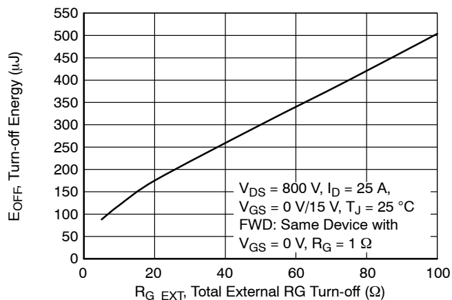
Figure 22. Clamped Inductive Switching Turn-Off Energy vs. R_{\text{G\_EXT\_OFF}}
