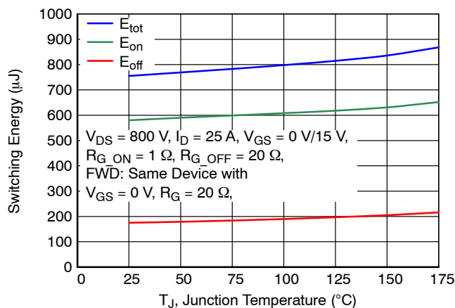
Figure 19. Clamped Inductive Switching Energy vs. Junction Temperature at V_{\text{DS}} = 800 \text{ V} and I_{\text{D}} = 25 \text{ A}
