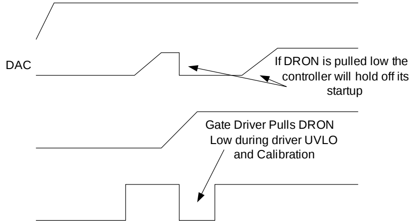
Figure 11. Gate Driver UVLO Restart
