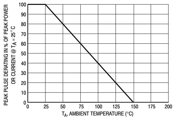
Figure 5. Pulse Derating Curve
