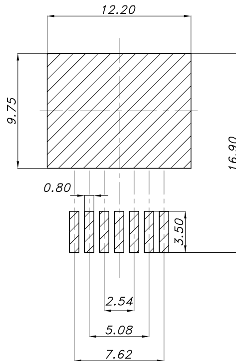
Figure 19. H 2 PAK-7 recommended footprint
