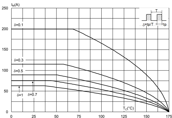
Figure 4. Peak forward current versus case temperature ( f_{sw} > 10 \text{ kHz} )
