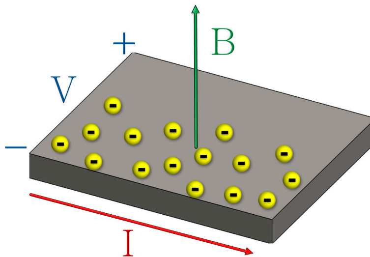
Figure 1-5. Hall-effect
