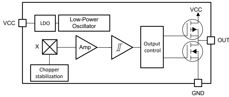
Figure 1-6. TMAG5233 Block Diagram
