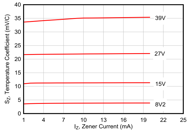
Figure 5-2. Temperature Coefficient
