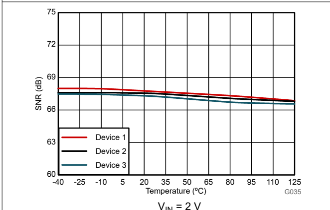
Figure 6-25. Signal-to-Noise Ratio vs Temperature
