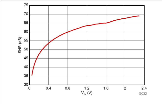
Figure 6-23. Signal to Noise Ratio vs Input Voltage
