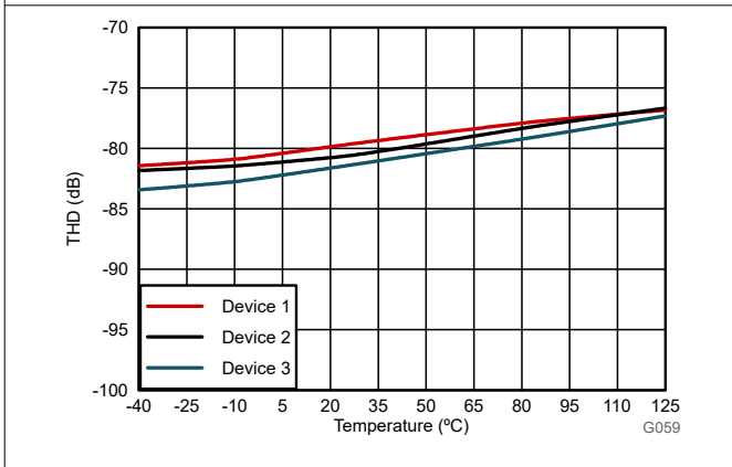
Figure 6-27. Total Harmonic Distortion vs Temperature
