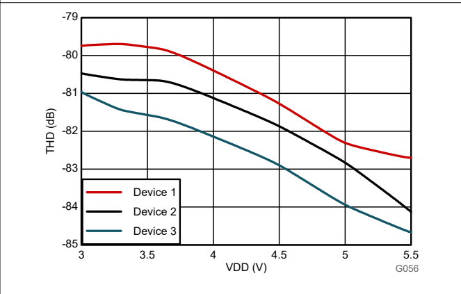
Figure 6-26. Total Harmonic Distortion vs Supply Voltage
