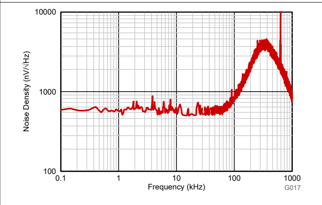
Figure 6-28. Input-Referred Noise Density vs Frequency
