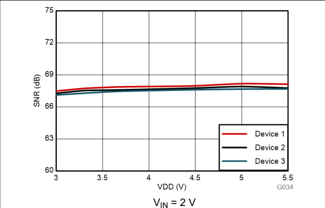
Figure 6-24. Signal-to-Noise Ratio vs Supply Voltage
