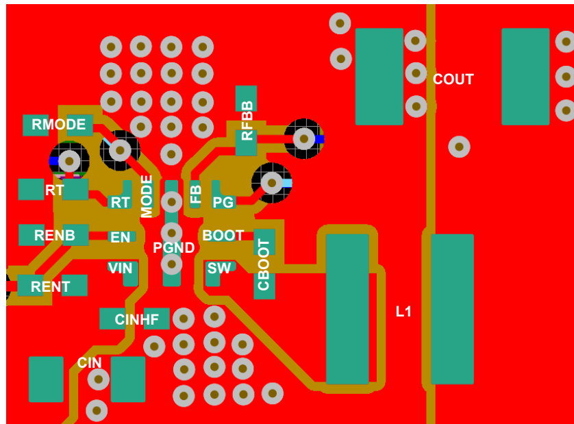
Figure 8-27. Fixed Output Version
