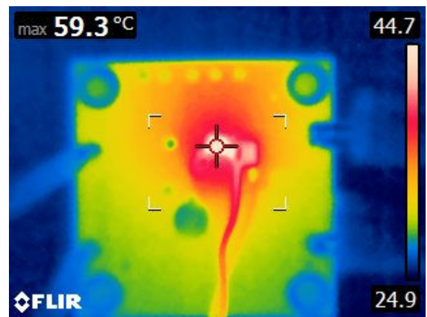
Device type = 3A 3.3V fixed output Mode = Auto F_{SW} = 2MHz
