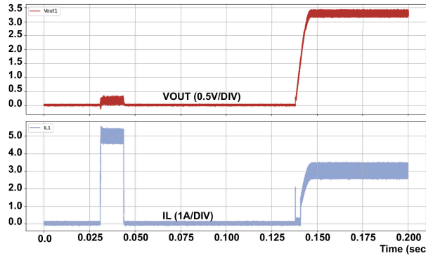
Device type = 3A 3.3V fixed output Mode = FPWM I_{OUT} = 3A F_{SW} = 2MHz
