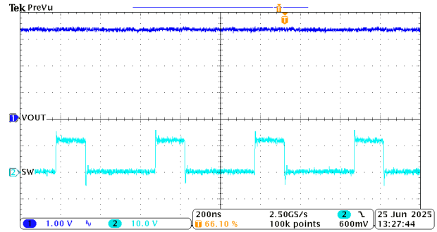
Device type = 3A 3.3V fixed output Mode = Auto I_{OUT} = 3A F_{SW} = 2MHz Continuous conduction mode
