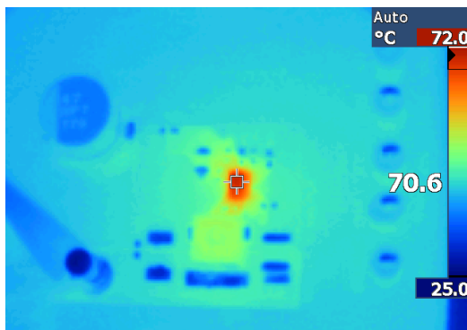
Device type = 3A 5V fixed output Mode = Auto F_{SW} = 2MHz
