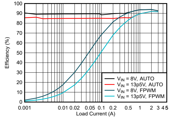
Device type = 3A 5V fixed output Mode = Auto/FPWM F_{SW} = 2MHz
