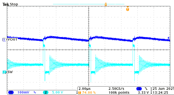
Device type = 3A 3.3V fixed output Mode = Auto I_{OUT} = 100mA F_{SW} = 2MHz Light load operation
