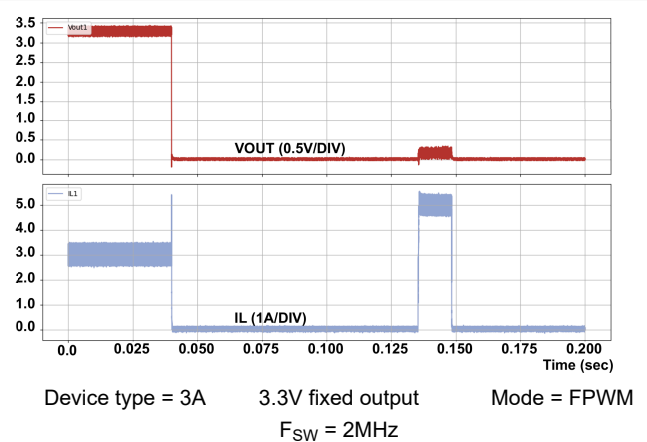
Figure 8-13. Short-Circuit Applied
