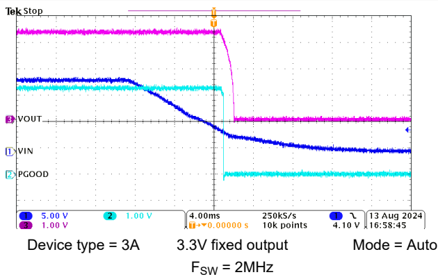
Figure 8-12. Shutdown Operation
