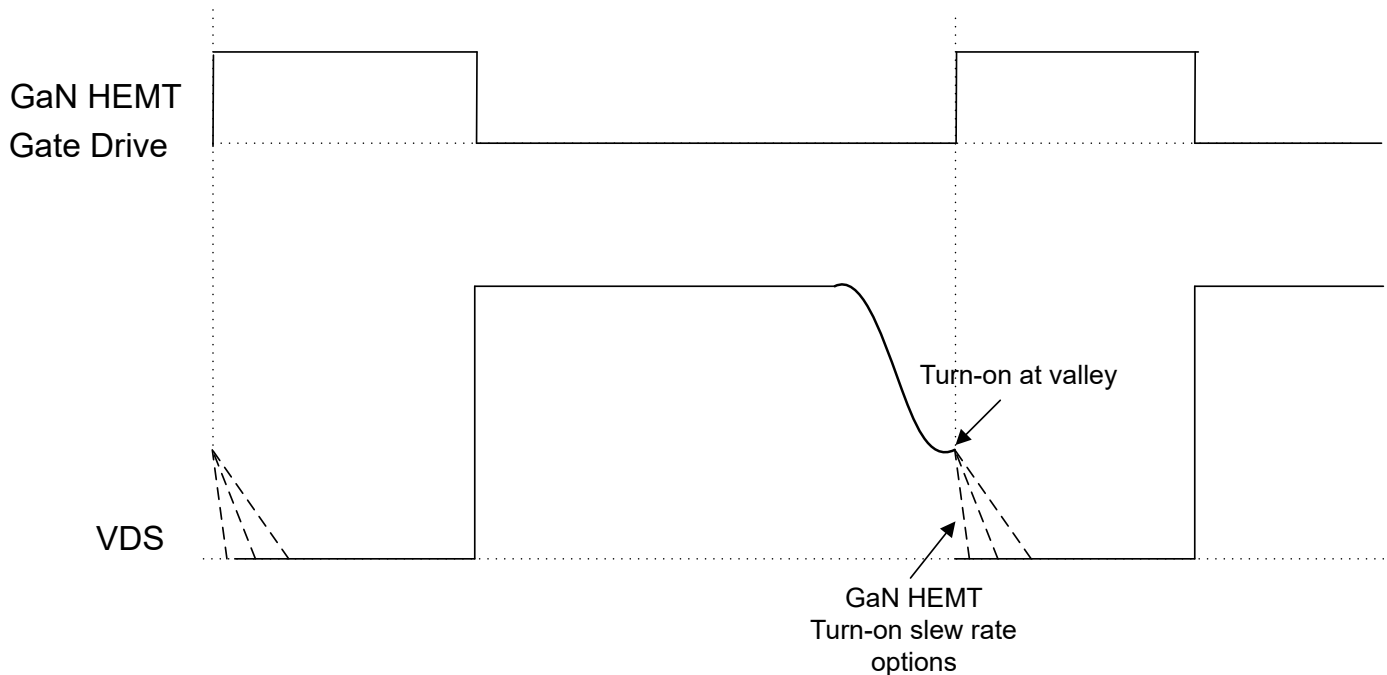
Figure 7-11. GaN HEMT Turn-On Slew Rate Control
