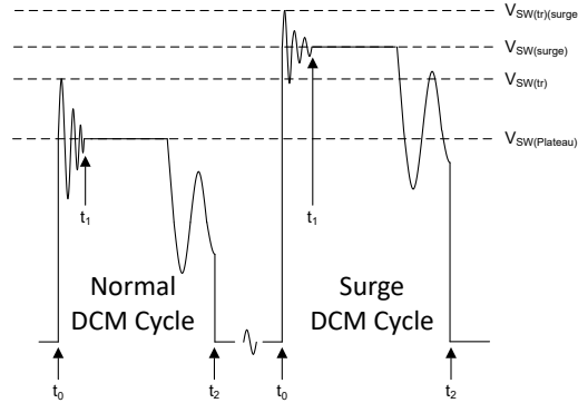
Figure 7-7. GaN HEMT Switching Capability
