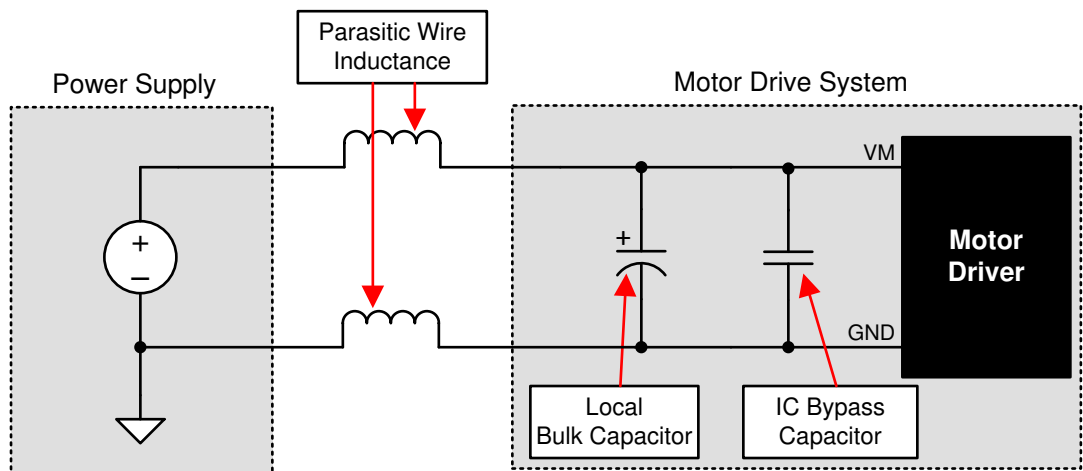
Figure 7-11. Example Setup of System With External Power Supply
