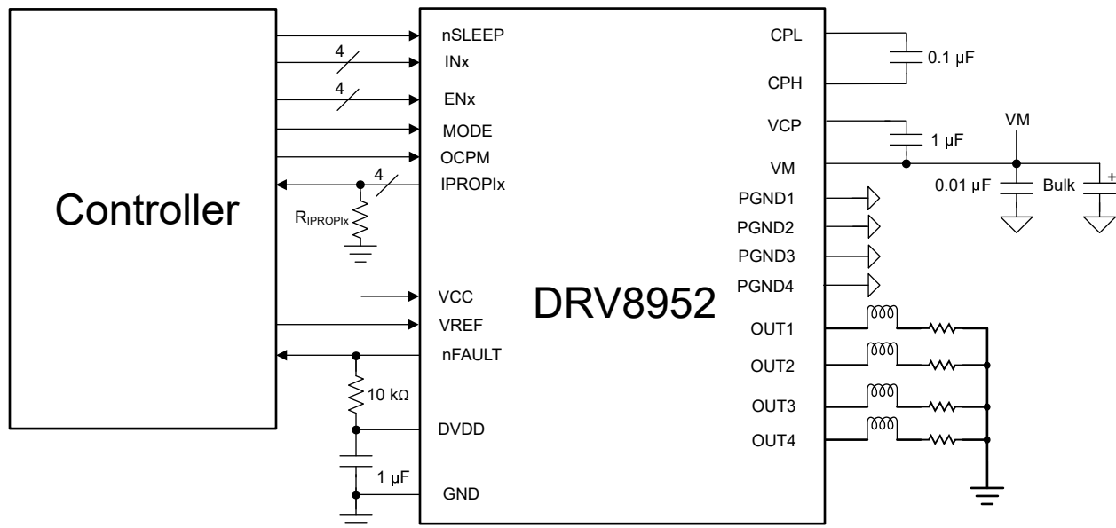
Figure 7-1. Driving Solenoids with DRV8952
