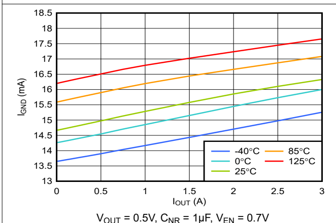
Figure 5-23. Quiescent Current vs I_{OUT}
