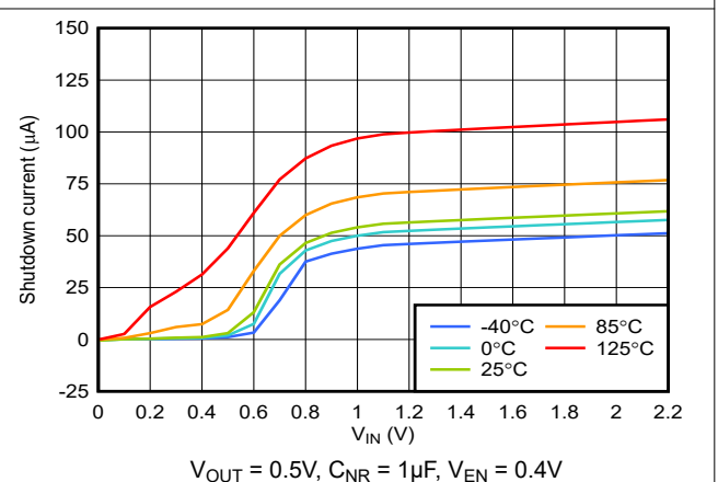
Figure 5-24. Shutdown Current vs V_{IN} for V_{OUT} = 0.5V
