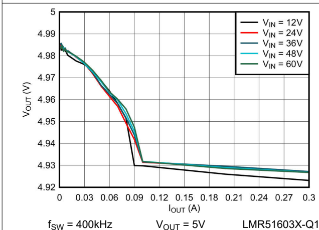
Figure 6-5. 5V load Regulation
