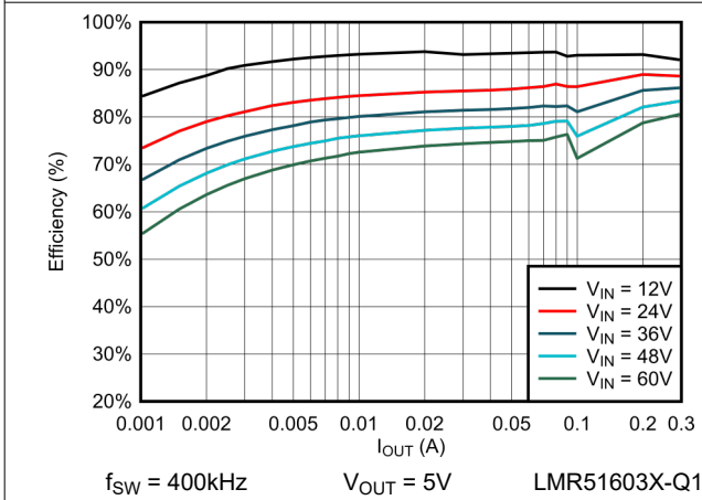
Figure 6-3. 5V PFM Efficiency Versus Load Current
