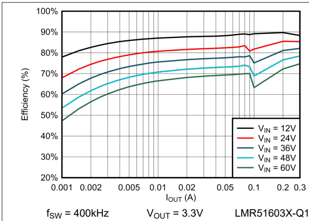
Figure 6-1. 3.3V PFM Efficiency Versus Load Current
