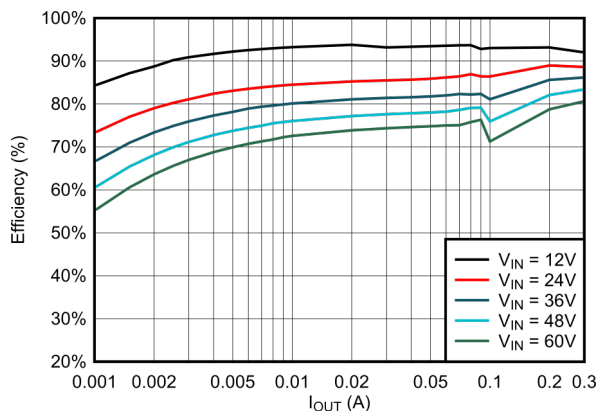
Efficiency Versus Output Current V_{OUT} = 5V, 400\text{kHz}
