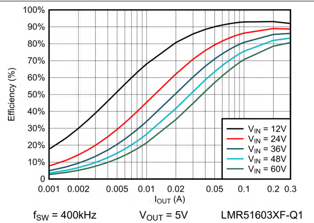
Figure 6-4. 5V FPWM Efficiency Versus Load Current
