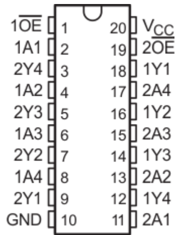
Figure 4-1. SN74LV8T240-Q1 PW or DGS Package; 20-Pin TSSOP or VSSOP (Top View)
