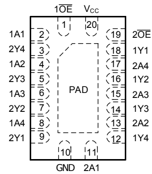
Figure 4-2. SN74LV8T240-Q1 RKS Package; 20-Pin TSSOP (Top View)
