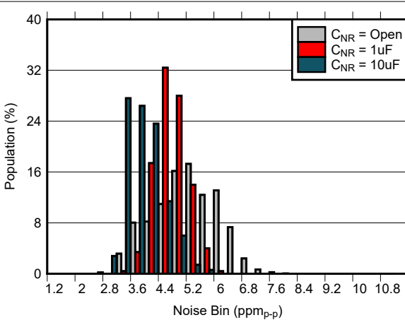
Figure 7-6. 0.1 Hz to 10 Hz Noise Distribution ( V_{REF} = 2.5\text{ V} , C_L = 1\ \mu\text{F} , I_L = 0\text{ mA} )
