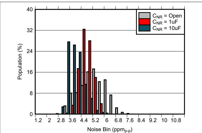
Figure 8-10. 0.1 Hz to 10 Hz Noise Distribution vs NR Capacitance
