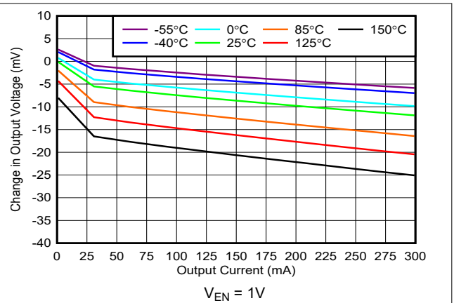
Figure 5-2. Load Regulation
