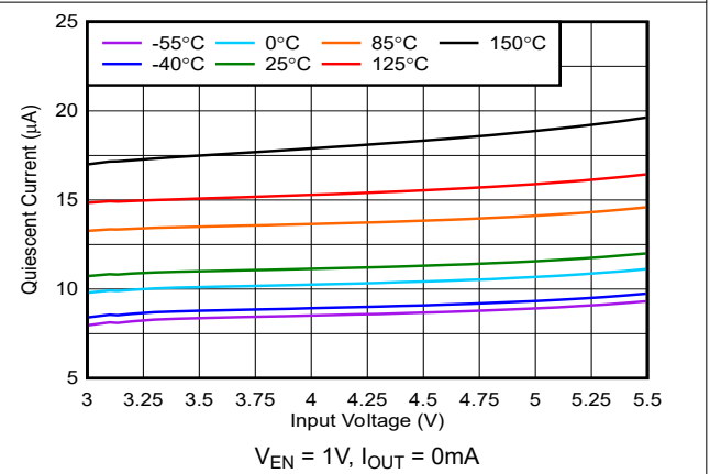
Figure 5-4. I_{GND} vs V_{IN}
