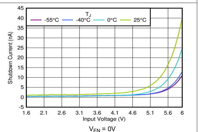
Figure 5-6. Shutdown Current vs V_{IN}
