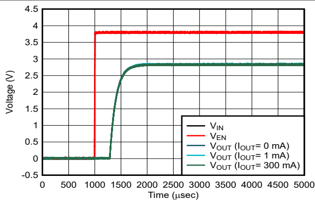
V_{IN} = V_{EN} = 0V to 3.85V , V_{IN} and slew rate = 1V/\mu s
