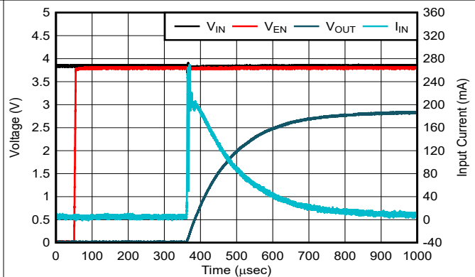
V_{IN} = 3.85V , V_{EN} = 0V to 3.85V , V_{EN} slew rate = 1V/\mu s , C_{OUT} = 10\mu F
