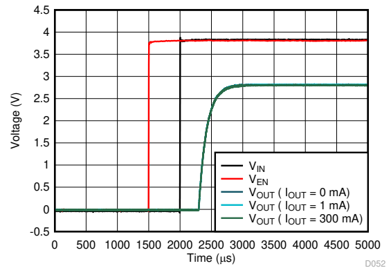
V_{IN} = 0V to 3.85V , V_{EN} = 0V to 3.85V , V_{EN} rises 500\mu s ahead of V_{IN} , V_{IN} and V_{EN} slew rate = 1V/\mu s
