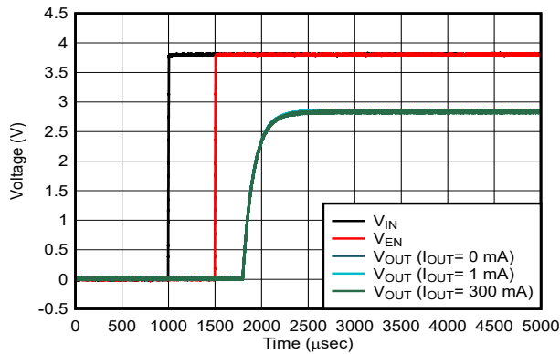
V_{IN} = 0V to 3.85V , V_{EN} = 0V to 3.85V , V_{EN} rises 500\mu s behind V_{IN} , V_{IN} and V_{EN} slew rate = 1V/\mu s
