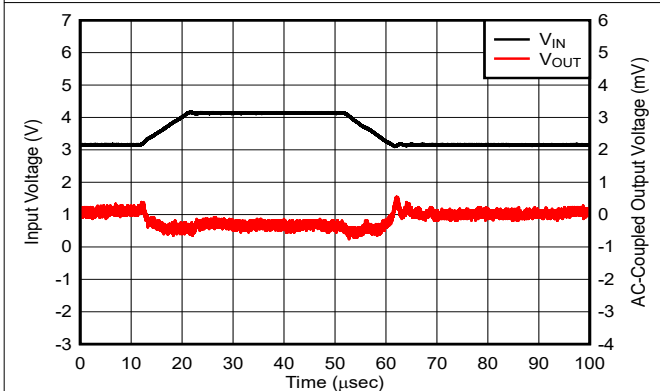
V_{IN} = 3.1V \rightarrow 4.1V \rightarrow 3.1V , V_{IN} t_{RISING} = 5\mu s , I_{OUT} = 150mA
