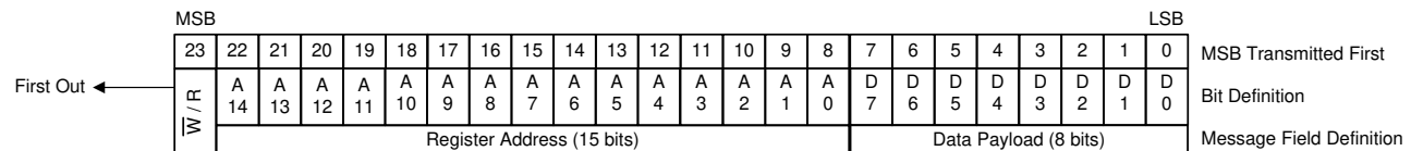
Figure 8-42. SPI Message Format
