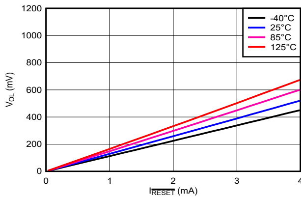
Figure 6-8. RESET Current (Sink) vs V_{OL} ( V_{DD} = 12\text{V} )
