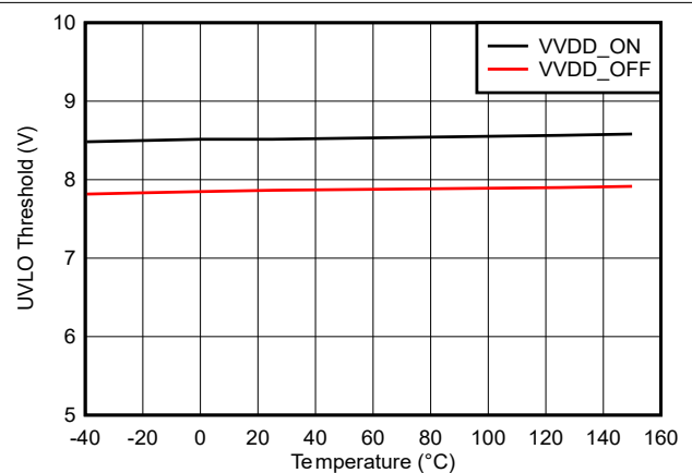
Figure 5-23. VDD 8-V UVLO Threshold vs Temperature
