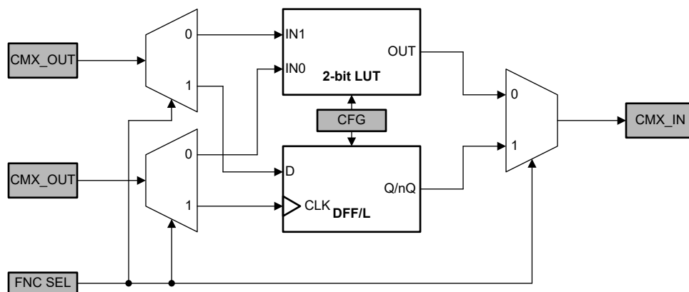
Figure 7-4. 2-bit LUT or DFF/Latch Block Diagram
