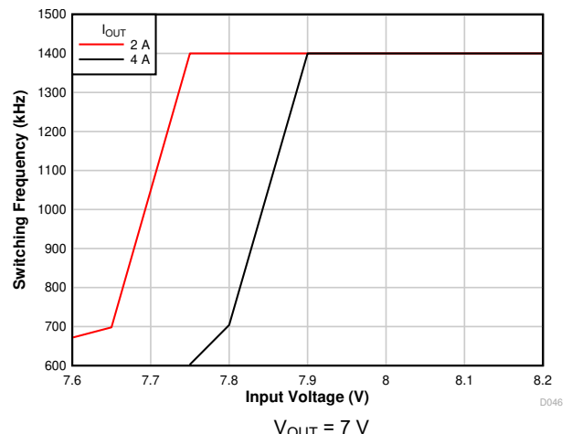
Figure 7-12. Frequency Foldback
