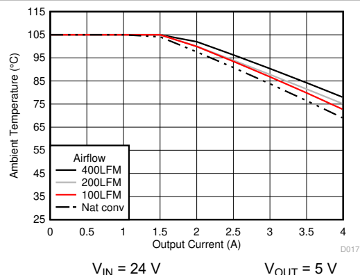
Figure 6-18. Safe Operating Area
