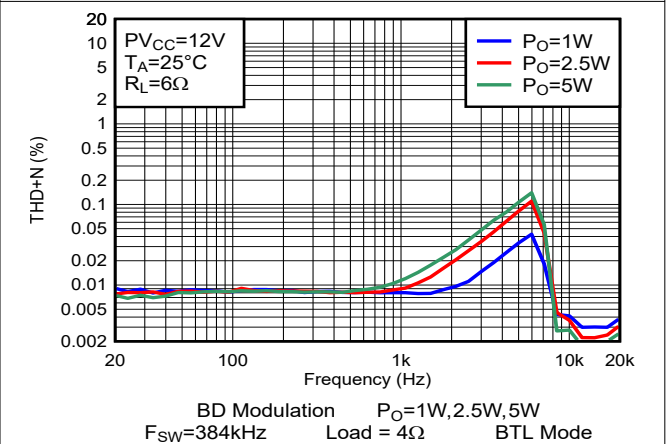
Figure 5-6. THD+N vs Frequency-BTL
