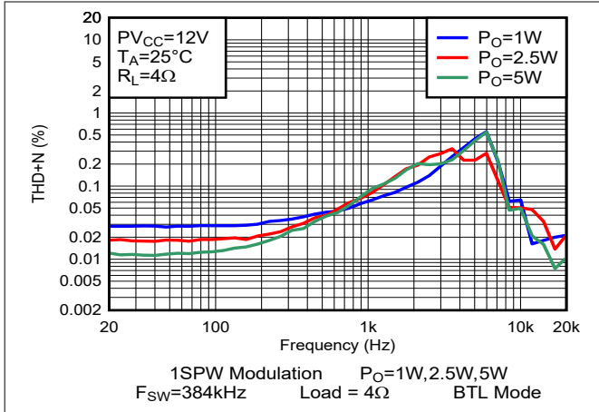
Figure 5-25. THD+N vs Frequency-BTL
