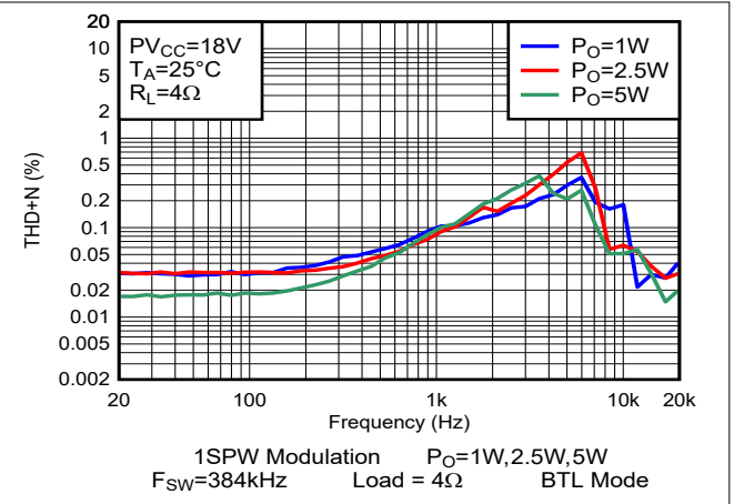
Figure 5-26. THD+N vs Frequency-BTL
