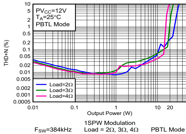
Figure 5-68. THD+N vs Output Power-PBTL
