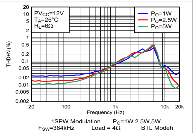
Figure 5-28. THD+N vs Frequency-BTL
