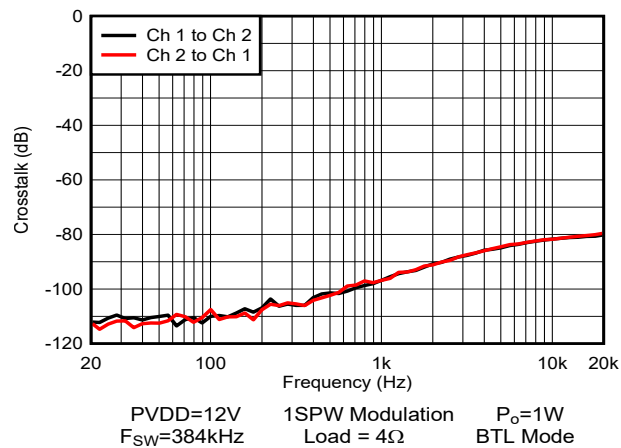
Figure 5-40. Crosstalk
