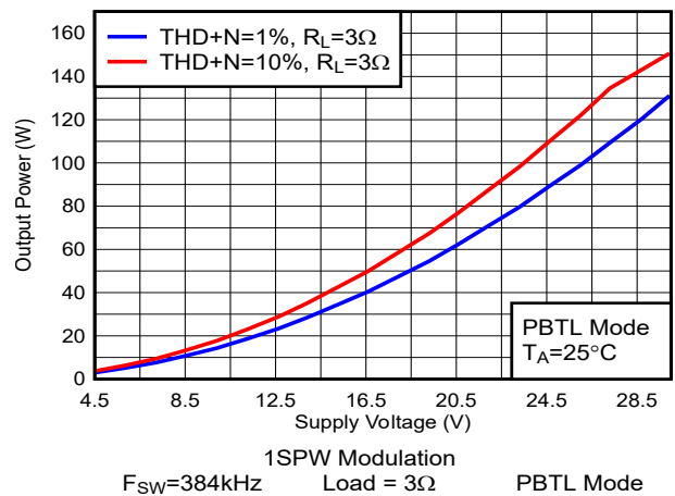
Figure 5-73. Output Power vs Supply Voltage
