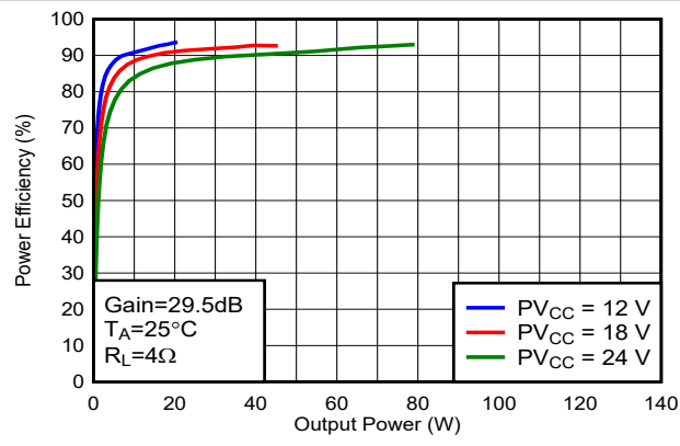
Figure 5-61. Efficiency vs Output Power
