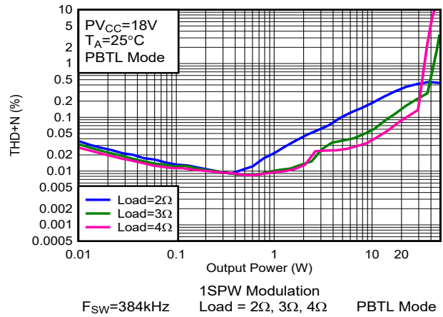
Figure 5-69. THD+N vs Output Power-PBTL
