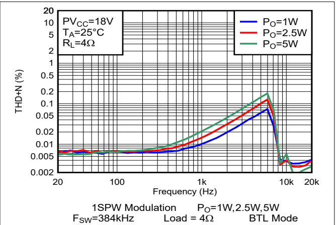
Figure 5-2. THD+N vs Frequency-BTL
