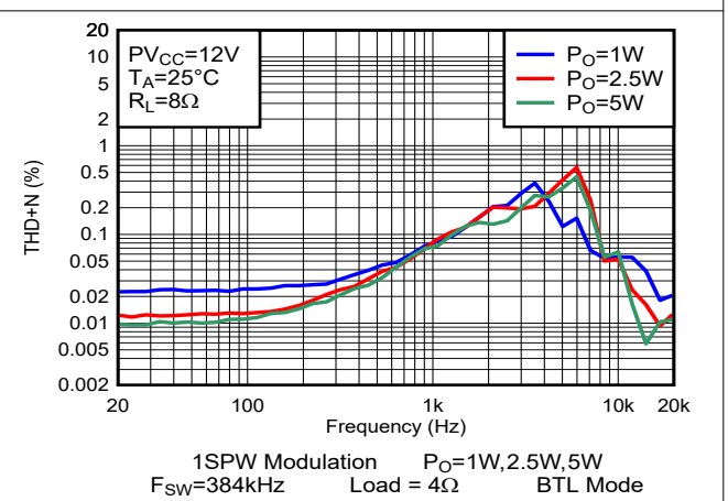
Figure 5-30. THD+N vs Frequency-BTL
