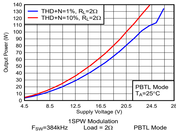
Figure 5-72. Output Power vs Supply Voltage
