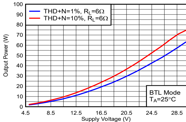
Figure 5-15. Output Power vs Supply Voltage
