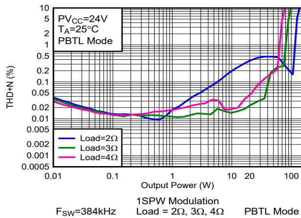
Figure 5-70. THD+N vs Output Power-PBTL
