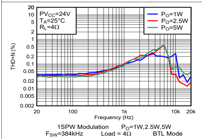
Figure 5-27. THD+N vs Frequency-BTL
