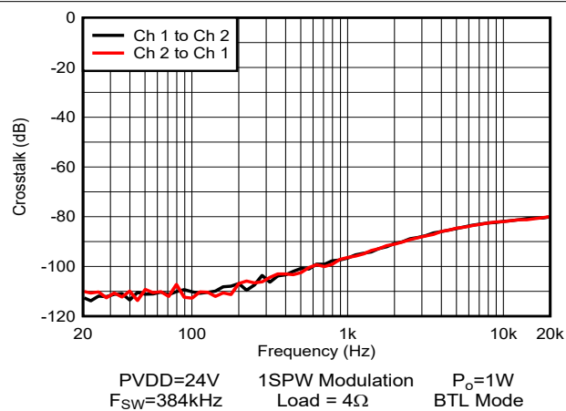
Figure 5-42. Crosstalk
