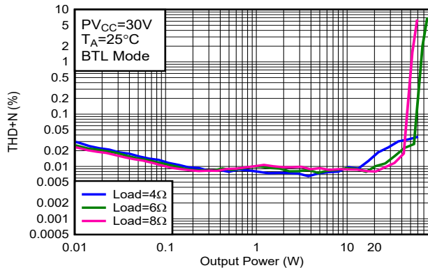
Figure 5-13. THD+N vs Power-BTL
