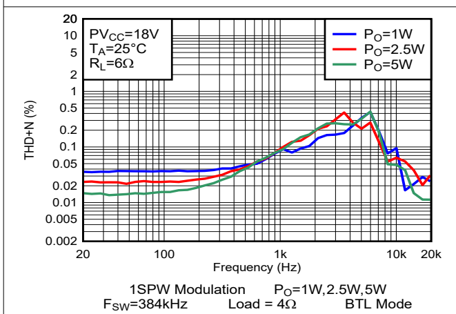
Figure 5-29. THD+N vs Frequency-BTL
