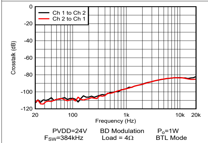
Figure 5-21. Crosstalk
