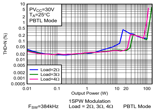
Figure 5-71. THD+N vs Power-BTL
