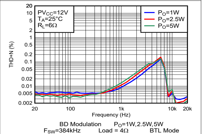
Figure 5-4. THD+N vs Frequency-BTL
