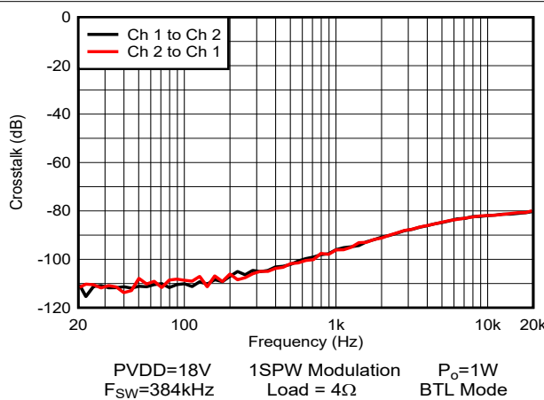
Figure 5-41. Crosstalk
