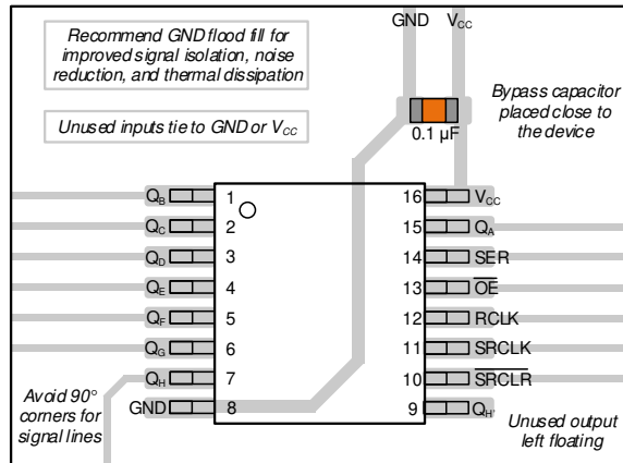
Figure 8-3. Example Layout for the SN74LV8T596-Q1 in TSSOP
