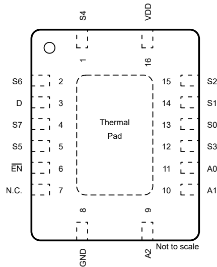
Figure 5-3. TMUX1308A-Q1: BQB Package, 16-Pin WQFN (Top View)
