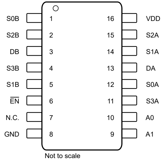
Figure 5-5. TMUX1309A-Q1: DYY Package, 16-Pin SOT-23-THIN (Top View)
