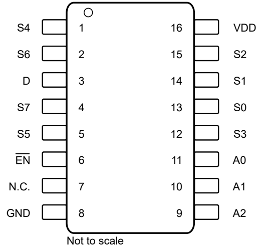
Figure 5-2. TMUX1308A-Q1: DYY Package, 16-Pin SOT-23-THIN (Top View)
