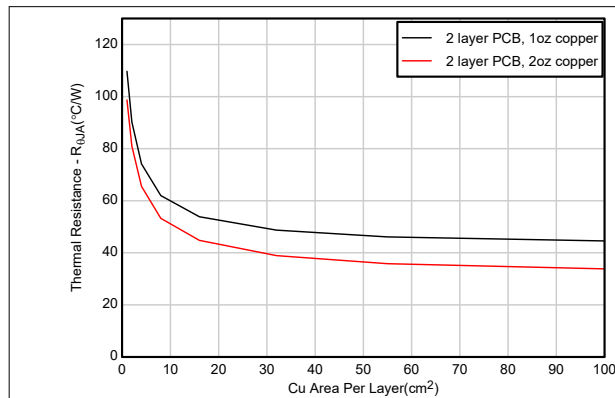
Figure 7-4. R_{\theta JA} vs Copper Area (HSOIC-8 Package, 2-layer PCB)
