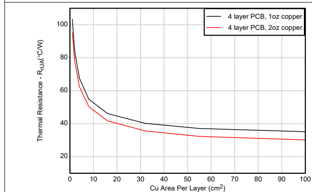
Figure 7-6. R_{\theta JA} vs Copper Area (HSOIC-8 Package, 4-layer PCB)
