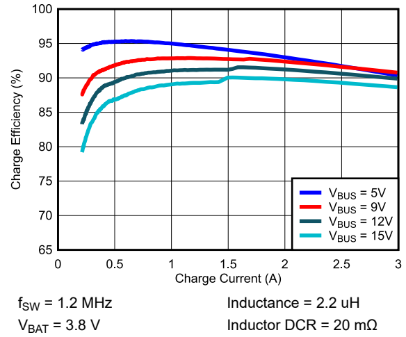
Figure 7-2. 1-Cell Battery Charge Efficiency vs Charge Current
