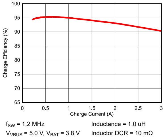
Figure 7-1. 1-Cell Battery Charge Efficiency vs Charge Current
